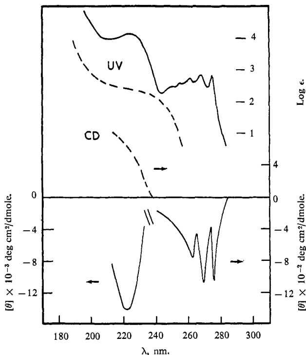
Figure 2. Ultraviolet and CD spectra of (-)-(1R,2R) -trans-1-methyl-2-phenylcyclopropane, (-) -2 (solid curves), and (-)-(1R,2R) -trans-2-methylcyclopropanecarboxylic acid, (-) -3 (dashed curves), in methanol solution. See ref 9 for explanation of the ordinate scales.
